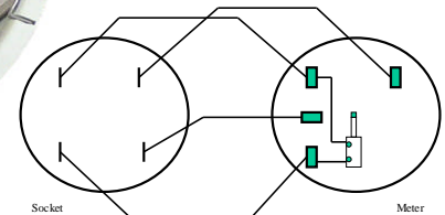
Both Meter & socket viewed from front, as if looking through meter.
